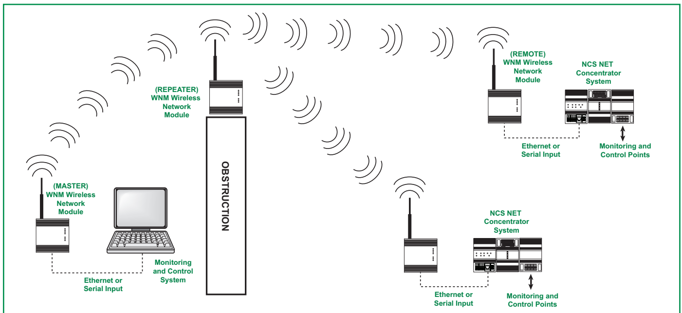
Figure 2. Point-to-Multipoint Mode
