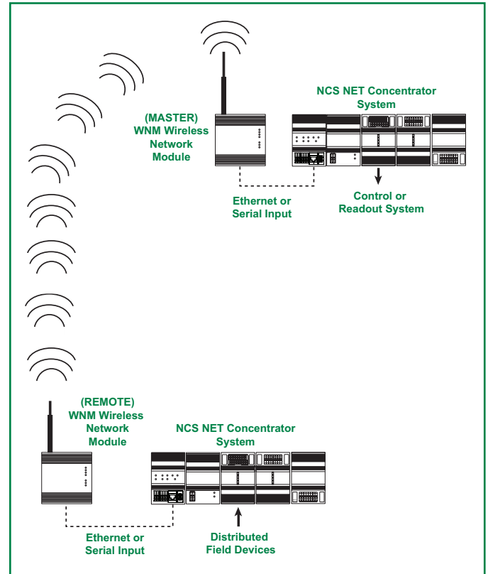
Figure 1. Point-to-Point Mode
