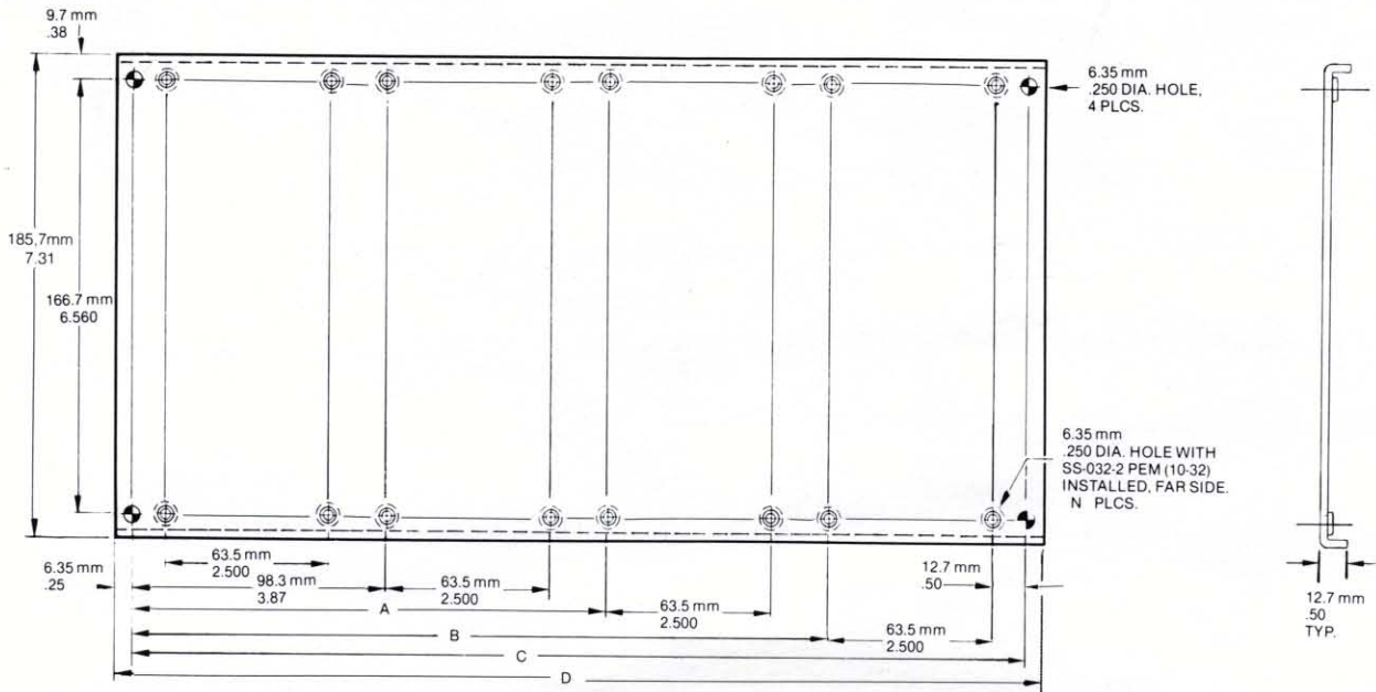
Figure 1. Standard Mounting Bracket for 2, 3, or 4 STD Housings
