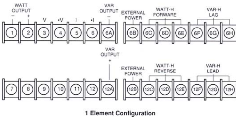
Figure 3. PCV Terminal Designations
