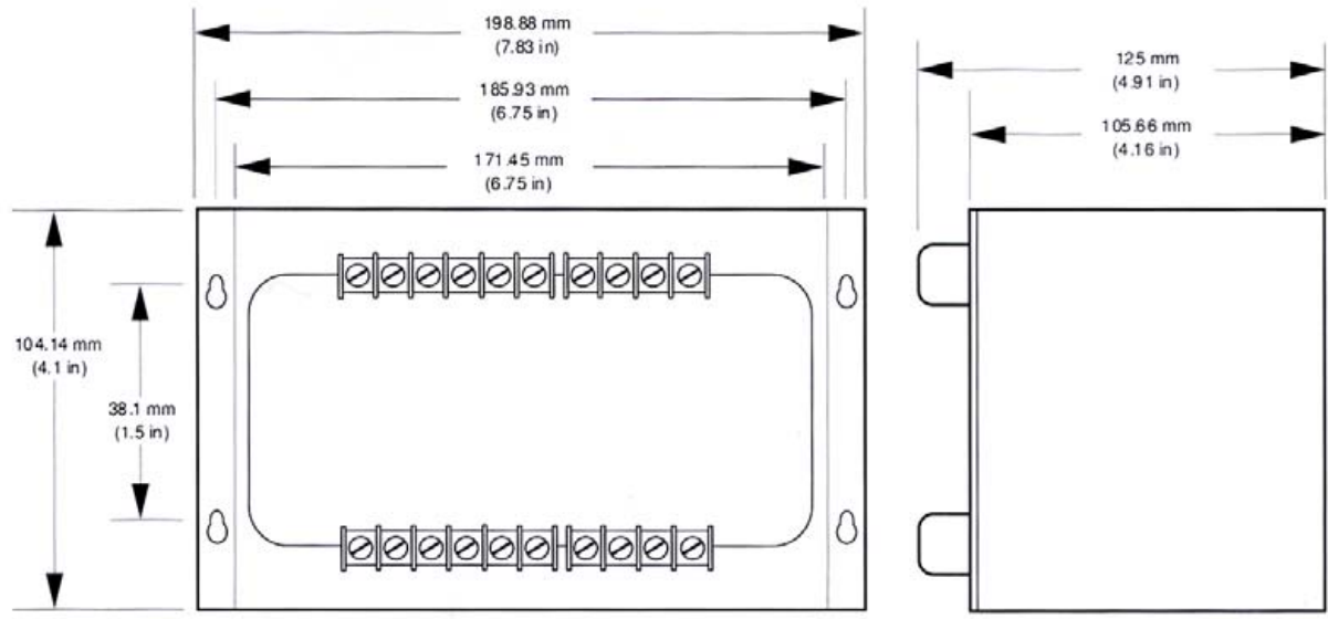
Figure 2. Outline Dimensions
