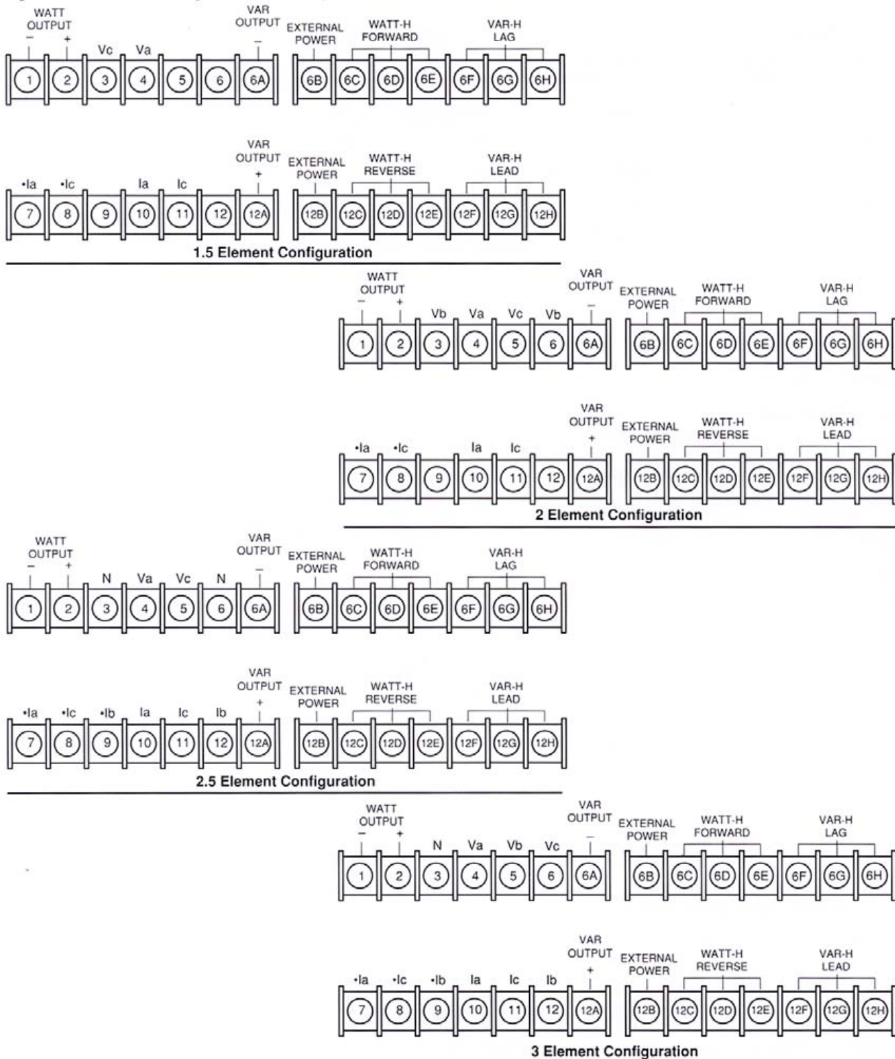
Figure 3. PCV Terminal Designations (continued)
