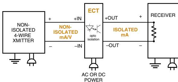
Figure 8. 4-wire ECT models are ideal for use where line (mains) power is readily available.
