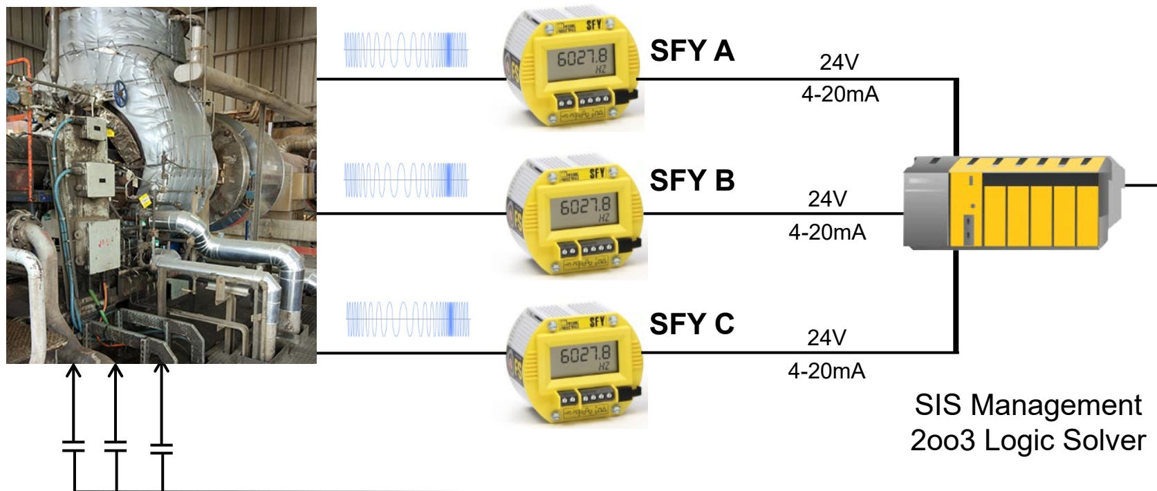
Overspeed Trips to Fan Blade Motor Control
