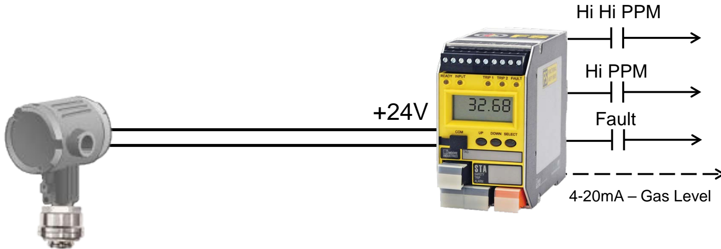
Gas Detector
