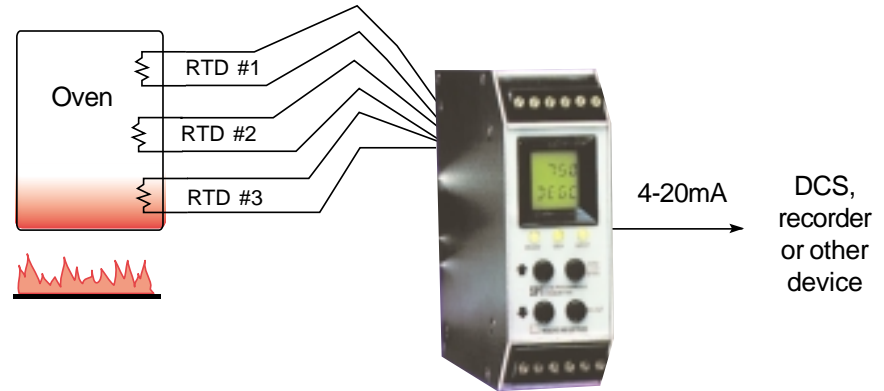
SPT Site-Programmable, Universal Temperature Transmitter
