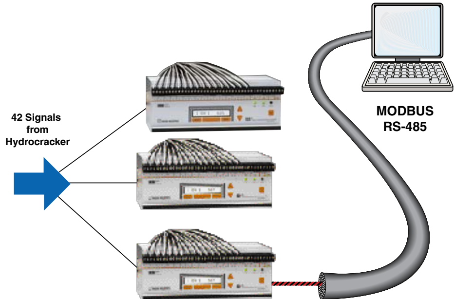
Three CCS Cable Concentrator Systems replace up to 48 isolators
